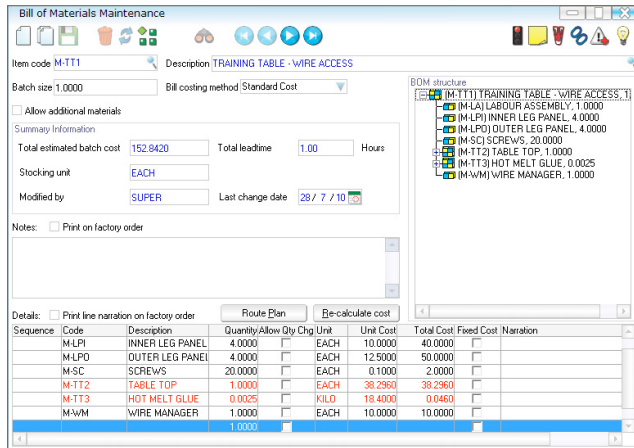
Multi-level Bill of Materials
